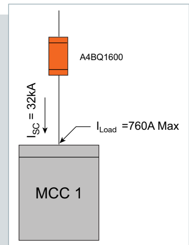
Figure 3: Single Line Diagram
